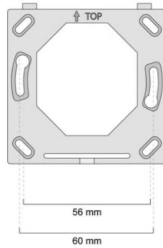
Fig.3. mounting plate
