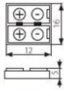
CONNECTOR 8
