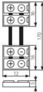
CONNECTOR 8-CPC
