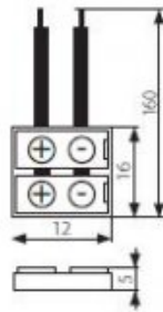
CONNECTOR 8-CP
