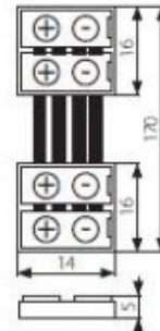
CONNECTOR RGB 10-CPC
